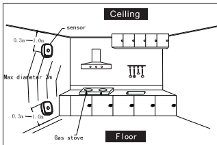
Mounting example
