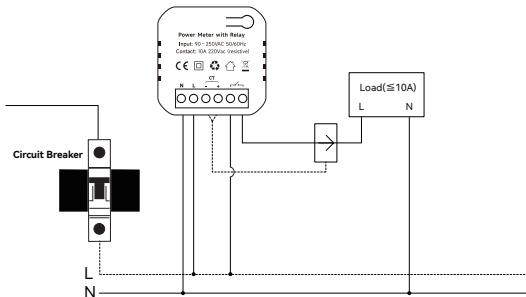
Wiring diagram
