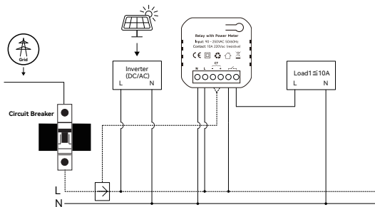
Wiring diagram
