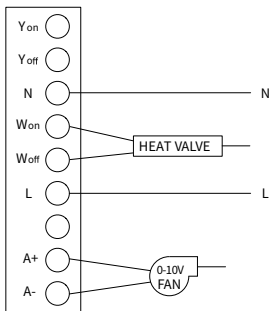
Two pipes Heat-only
