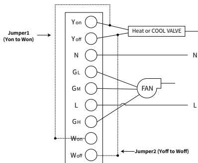
Two way valve
