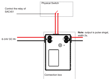
Installation diagram
