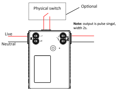
Wiring diagram
