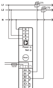
Split Phase, Wiring
