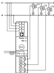
Single Phase, Three Loads Wiring
