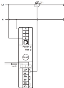
Single Phase, One Circuit Wiring
