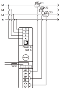
Three Phase Four Wire, Wiring
