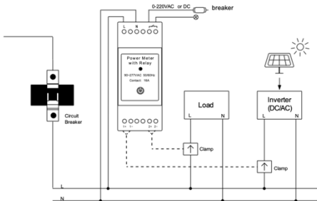
Single phase electricity wiring diagram
